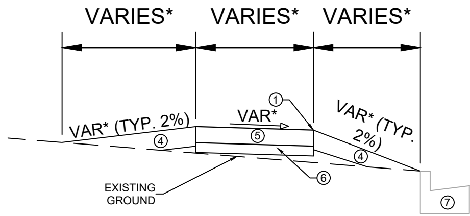
TYPICAL SECTION BARTILLON PATH (STA 59+25 TO STA 59+50)
